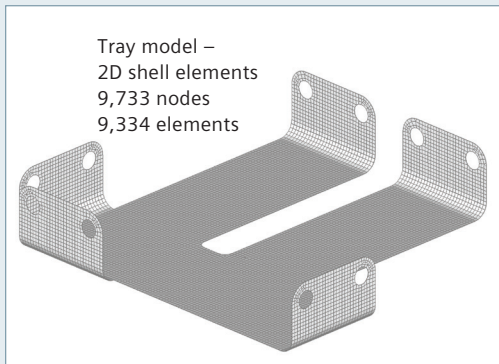
Figure 5: Thin walled model size comparison.
