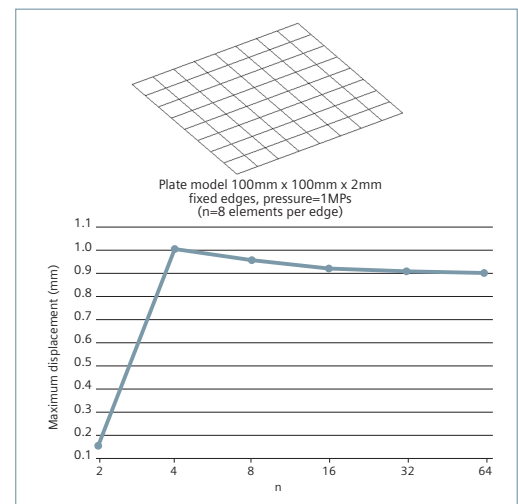
Figure 3: Mesh convergence analyses can help determine the required model size to ensure accurate results.
