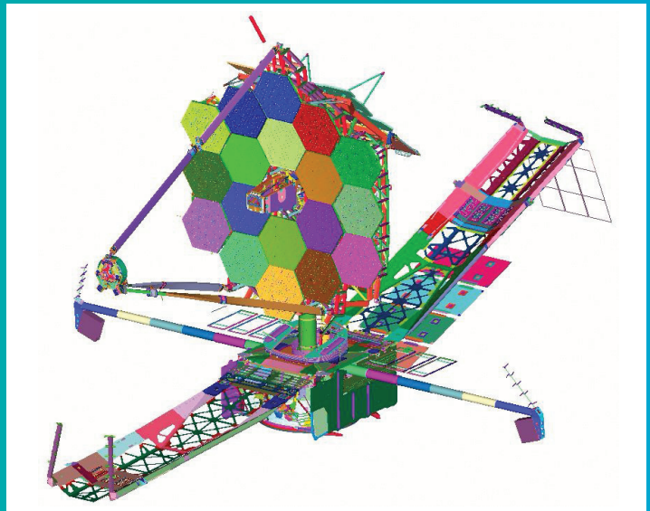
NASA Goddard Space Flight Center – James Webb Space Telescope Femap model courtesy of SGT Inc.
